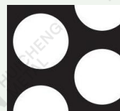
7/16" Diameter 9/16" Centers 51% Open Area
