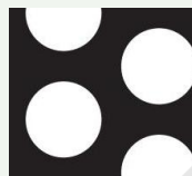
3/8" Diameter 9/16" Centers 40% Open Area
