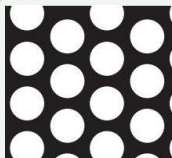
3/16" Diameter 1/4" Centers 51% Open Area
